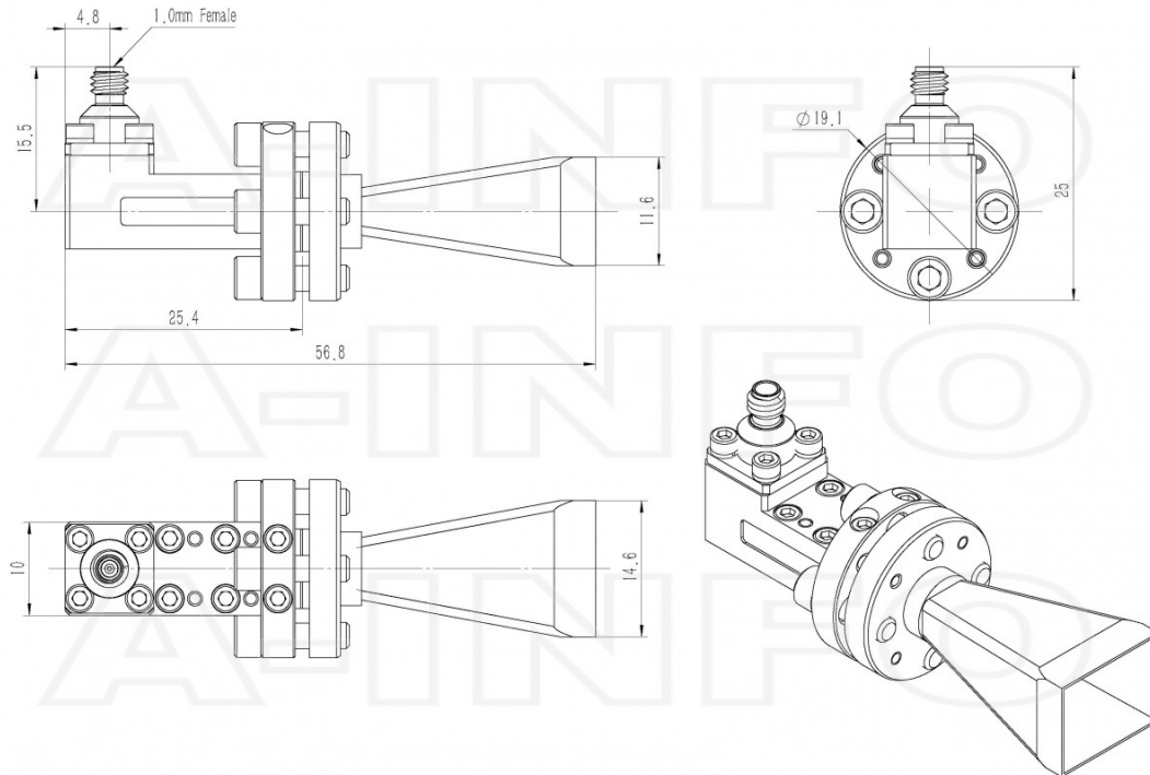
1.0mm-Female Output (P/N: LB-10-20-C-1.0F)
